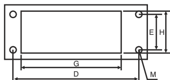
Panel Cutout
